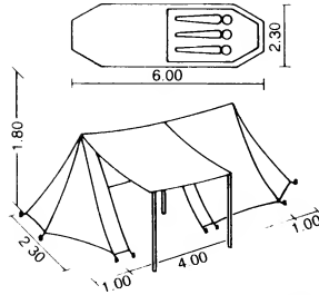
2 With inner tent, two awnings and canopy
